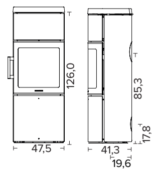
HWAM 3130m with traditional handle
