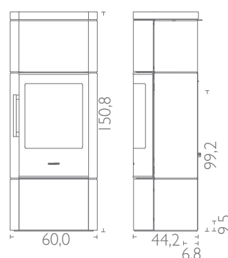
HWAM 3660m with soapstone cladding
