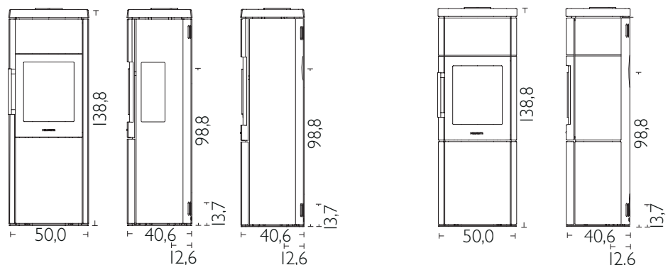
HWAM 4550m with side glass
