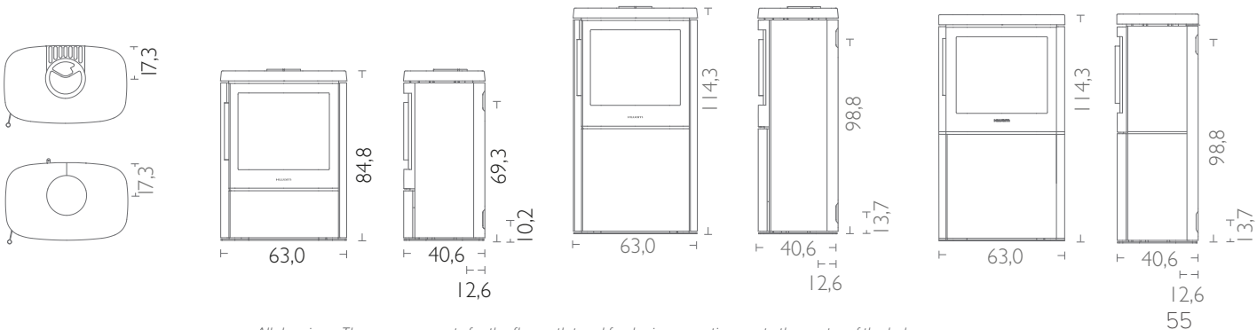
HWAM 4640m with soapstone cladding
