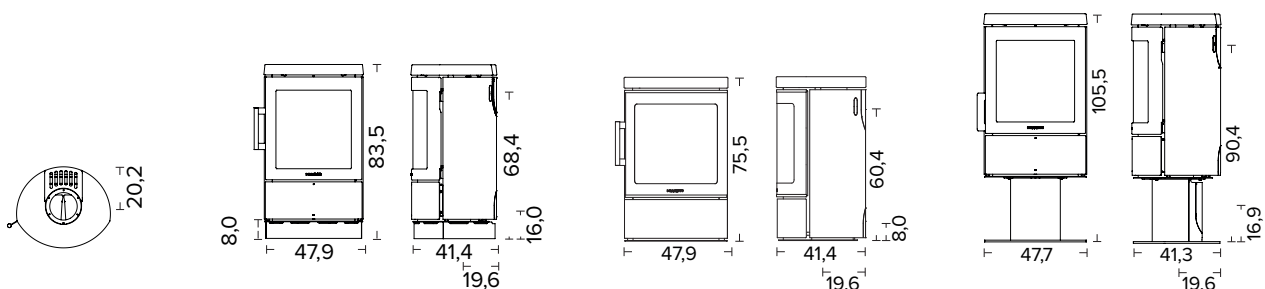
HWAM 3110c on a pedestal & with style handle, black
