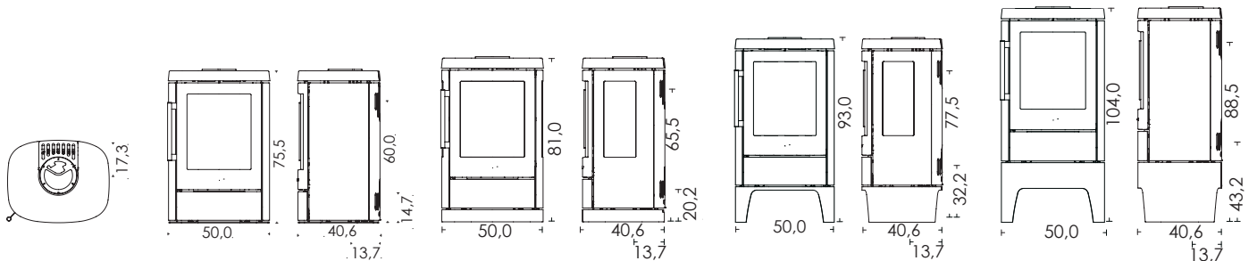
HWAM 4510c with side glass & on a low base HWAM® Autopilot™
