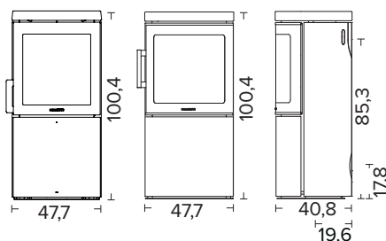
HWAM 3120c with style handle, stainless steel
