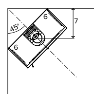
HWAM Classic 4
