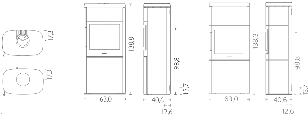
HWAM 4660m with Tobacco stone cladding
