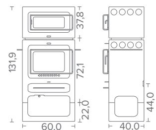
HWAM Classic 4 with baking oven and wood store
